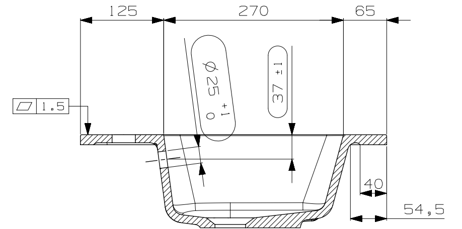
SECTION F-F SCALE 35:200
