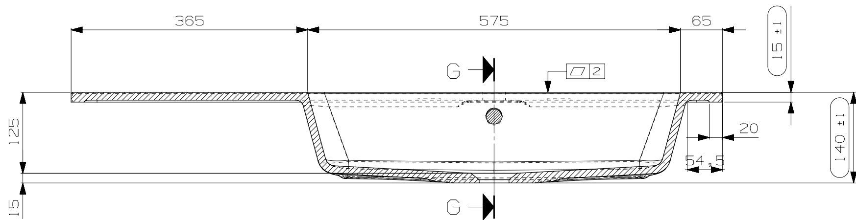
SECTION H-H SCALE 35:200
