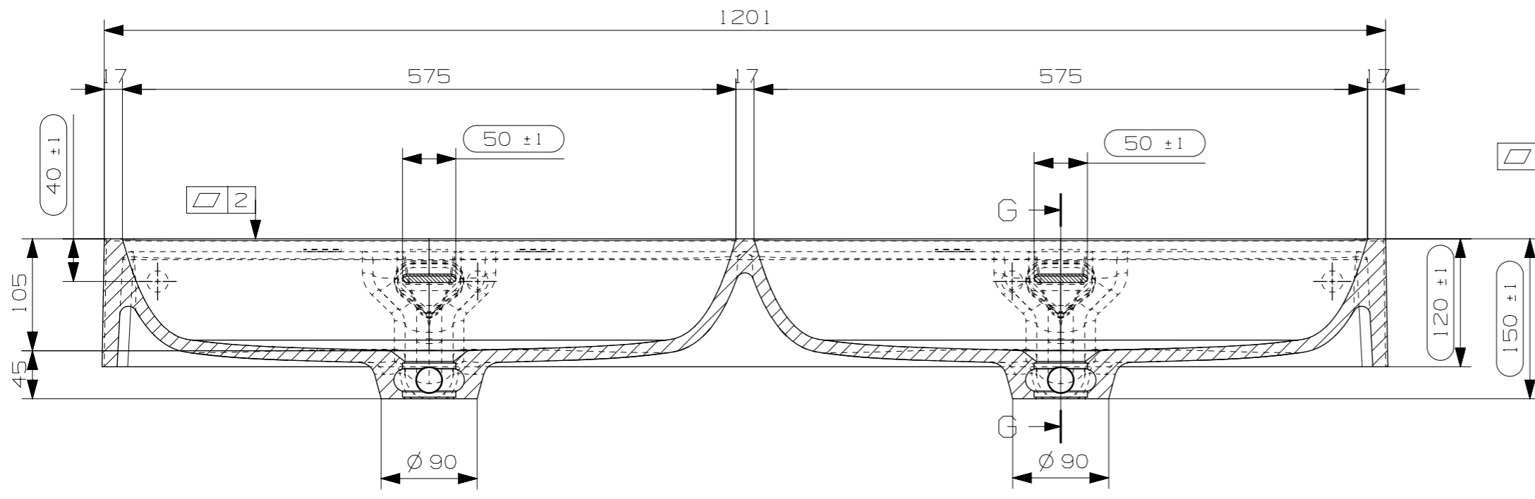
SECTION F-F SCALE 1:5
