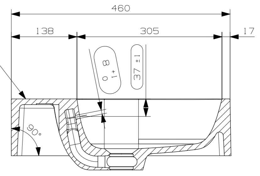
SECTION G-G SCALE 1:5
